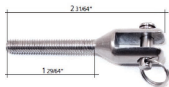
Threaded Fork Stud
