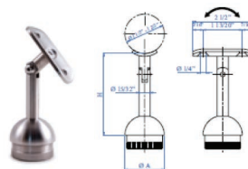
Adj. Handrail support (post)
