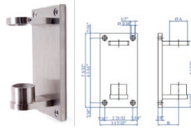
B528 Fits 1.67" dia B = 1.94"
