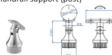
Adj. Handrail support (post)
