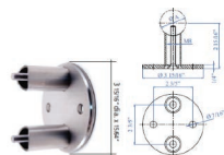
B524 Fits 1.67" dia
