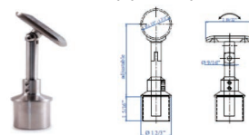
Adj. Handrail Support (post) w/Adj. Height
