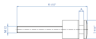
B640 Glass 0.625" to 0.875"
