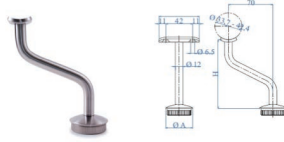
Handrail Support (post)
