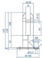
Floor and Wall clamp w/ Flange
