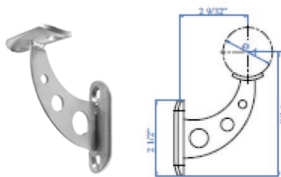
B219 A = 1.67" dia
