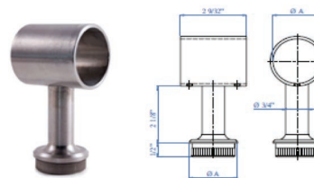
Handrail support (post) thru
