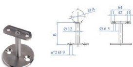
Flanged Handrail Support
