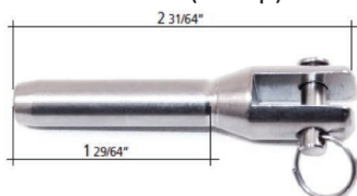
Terminal Fork (Crimp)
