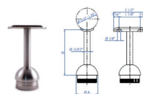
Handrail support (post)
