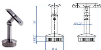
Adj. Handrail Support (post)
