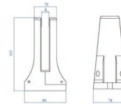
B641, M641 A = 0.53" & 0.69" / 13.52mm, 17.52mm
