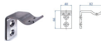
B223 For Round Tube
