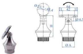
Adj. Handrail Support (post)
