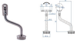
Adj. Handrail Support (post)
