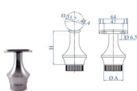
Handrail Support (post)
