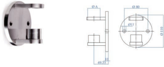
B527 Fits 1.5", 1.67", 2" dia.
