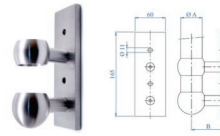
B529 Fits 1.33", 1.67" B = 2.44"
