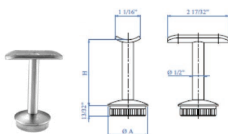
Handrail Support (post)
