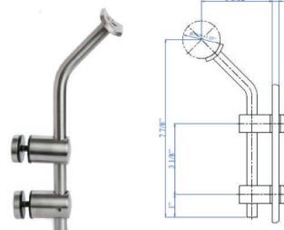
B642 Glass 0.3125" to 1" Drill at 0.86" dia
