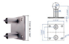
B525 Fits 1.67" dia
