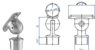
Adj. Handrail support (post)
