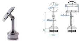
Adj. Handrail Support (post)
