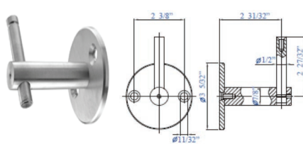
B220 (Round Saddle Included) Fits 1.33" – 1.67" dia Removable Saddle
