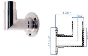
B258 A = 1.67" dia
