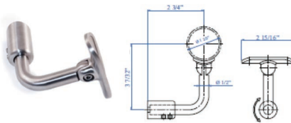
B218 Fits 1.67" dia tube
