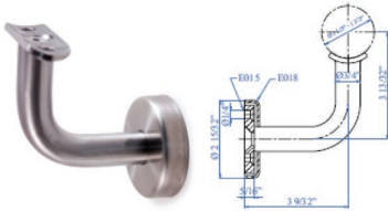
B215 Fits 1.33" – 1.67" dia Removable Saddle
