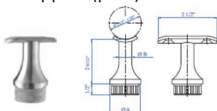
Handrail Support (post)
