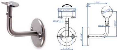
B213, M213 Fits 1.33" – 1.67" dia Removable Saddle
